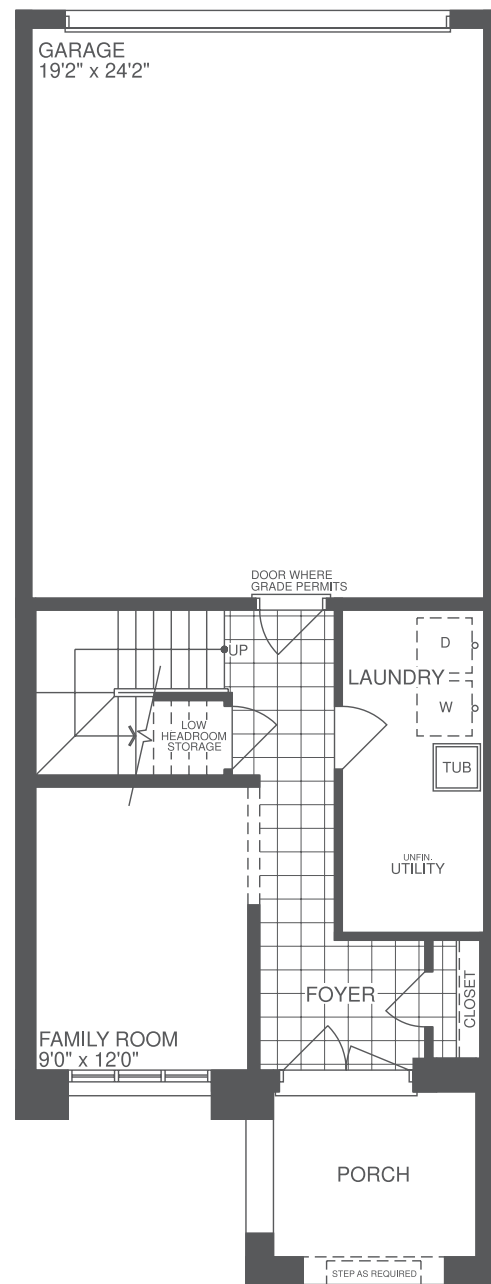
GROUND FLOOR ELEVATION A 1750 sf
