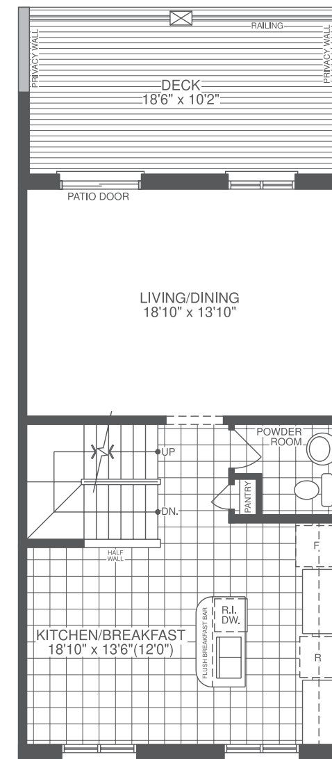
MAIN FLOOR ELEVATION A 1750 sf
