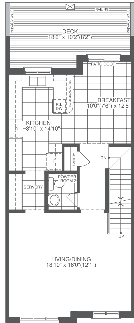
MAIN FLOOR ELEVATION A 2002 sf
