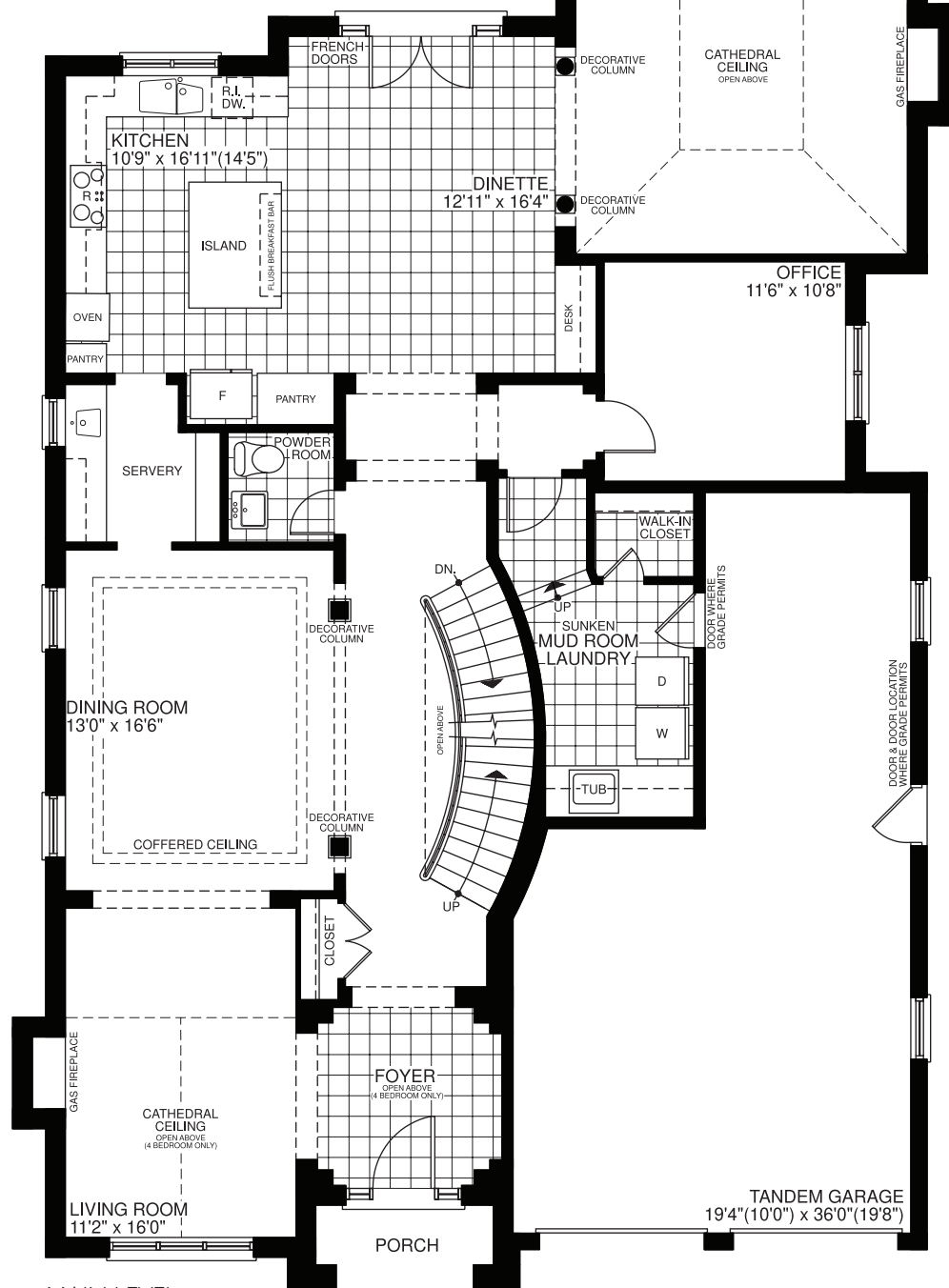
MAIN LEVEL
