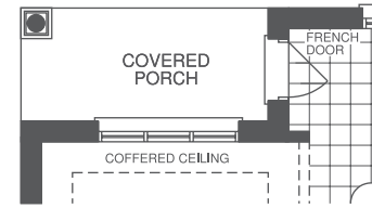
MAIN FLOOR REAR ELEVATION C 2318 sf
