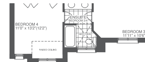
SECOND FLOOR 4 BEDROOM + DEN ELEVATION B 2729 sf
