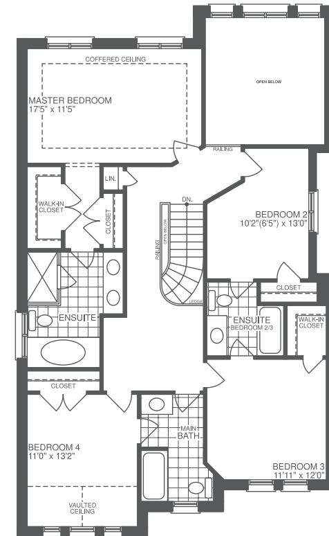
ALT. SECOND FLOOR ELEVATION A 2578 sf
