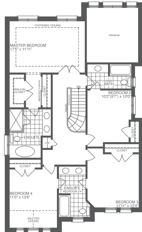
SECOND FLOOR ELEVATION A 2584 sf
