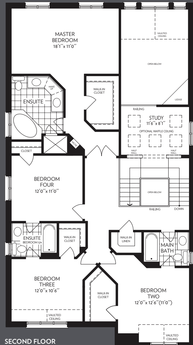
SECOND FLOOR 4 BEDROOM ELEVATION B
