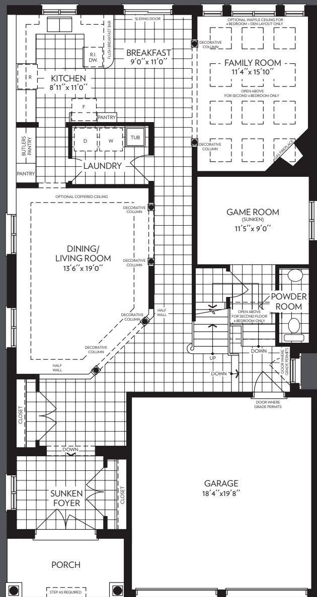
FIRST FLOOR ELEVATION B
