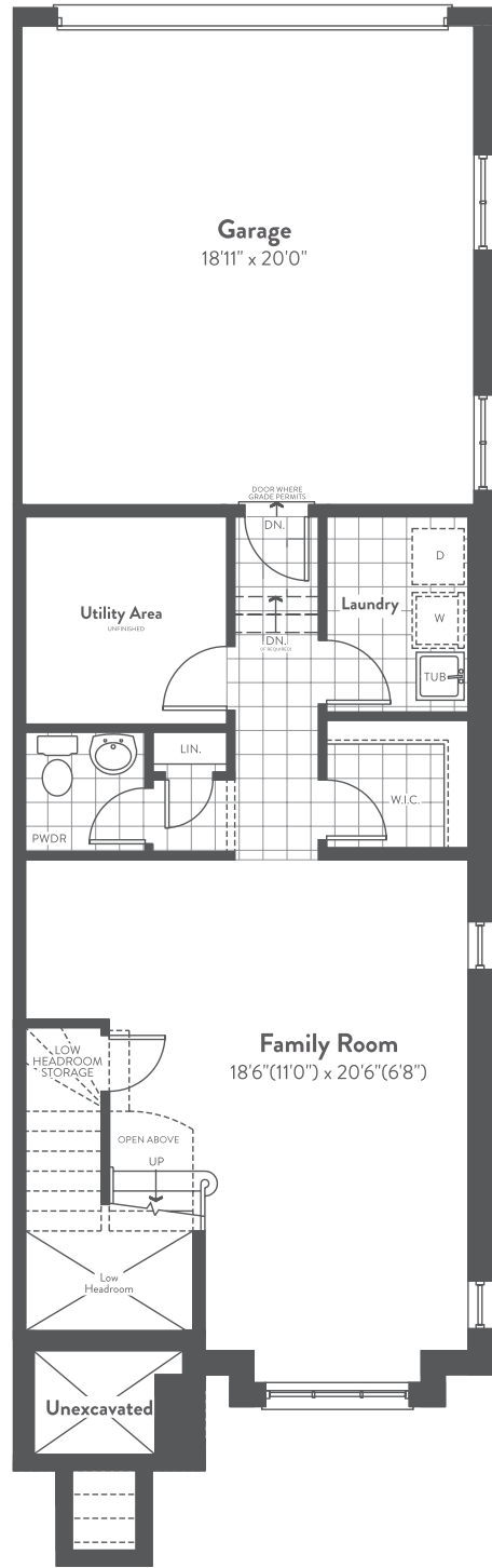
LOWER FLOOR ELEV. B-2
