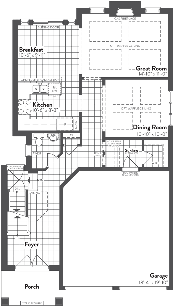
FIRST FLOOR ELEVATION A 2075 sf
