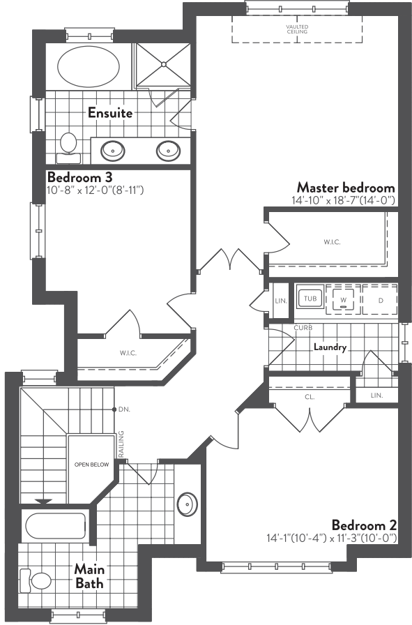
SECOND FLOOR ELEVATION A 2075 sf
