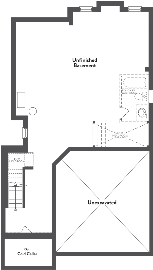
BASEMENT ELEVATION A/B/C 2075/2085/2091 sf
