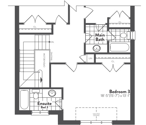
SECOND FLOOR ELEVATION C
