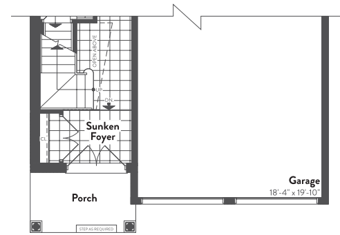
FIRST FLOOR ELEVATION B
