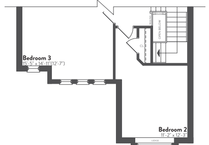
SECOND FLOOR (4 BEDROOM) ELEVATION C
