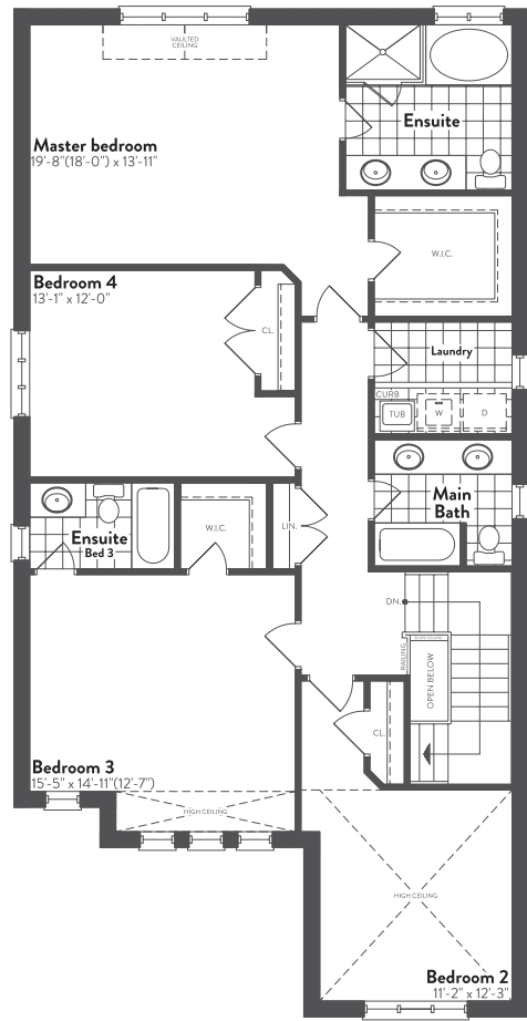
SECOND FLOOR (4 BEDROOM) ELEVATION A
