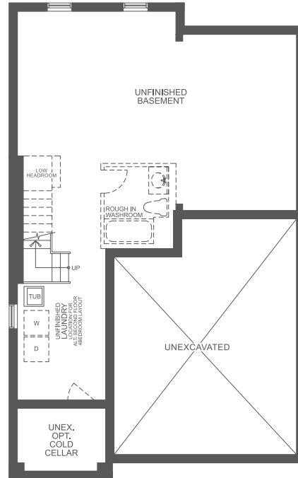
UNFINISHED BASEMENT ELEVATION A 2019 sf
