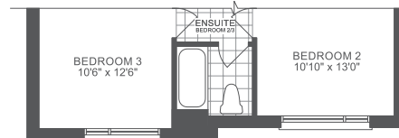
SECOND FLOOR PLAN 3 BEDROOM ELEVATION C 2009 sf
