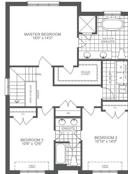
SECOND FLOOR PLAN 3 BEDROOM ELEVATION A 2019 sf
