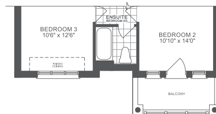
SECOND FLOOR PLAN 3 BEDROOM ELEVATION B 2019 sf
