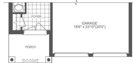
MAIN FLOOR PLAN ELEVATION B 2019 sf
