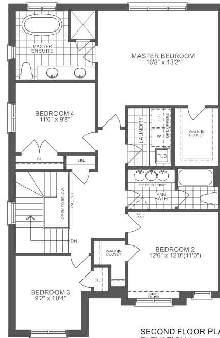
SECOND FLOOR PLAN ELEVATION A 2212 sf
