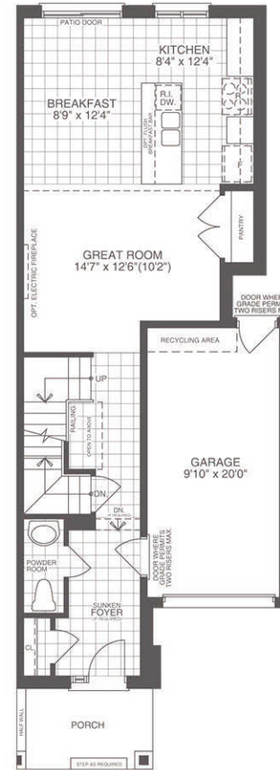
OPT. GROUND FLOOR PLAN ELEVATION A 1602 sf
