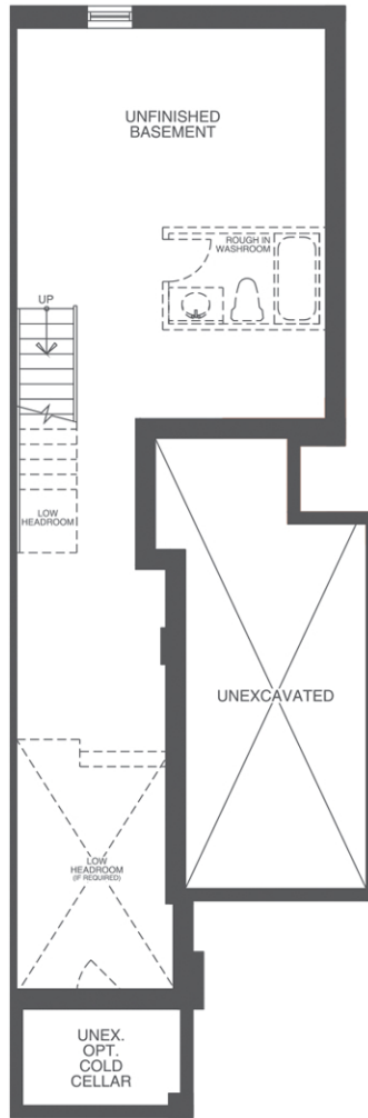
UNFINISHED BASEMENT ELEVATION A & A1 1715 sf
