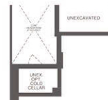
UNFINISHED BASEMENT/ 401 sf OF OPT. FINISHED BASEMENT ELEVATION B 1763/2164 sf
