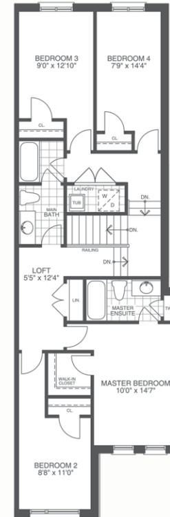
OPT. SECOND FLOOR PLAN 4 BEDROOM ELEVATION A 1966 sf
