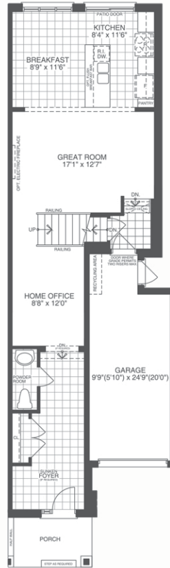
GROUND FLOOR PLAN ELEVATION A 1966 sf
